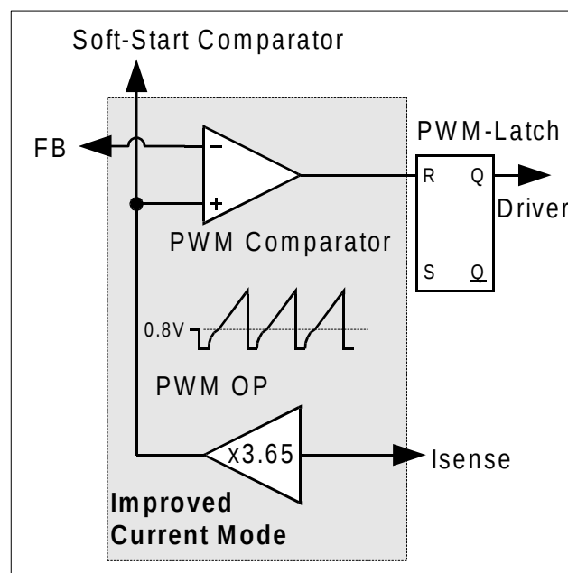
Figure 7 Current Mode
